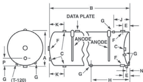
FIGURE 1 -T-80, T-120 NOTE:T-120 SHOWN.
