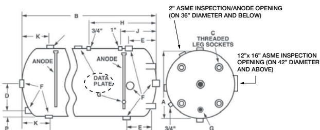
FIGURE 2 - T-140 THRU T-1000A
